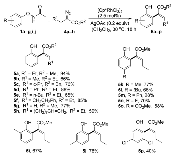
Scheme 5. Scope of diazoesters and N -phenoxyacetamides. Reaction conditions: 1 (0.30 mmol), 4 (0.33 mmol), [\text{Cp}^*\text{RhCl}_2]_2 (2.5 mol%), and AgOAc (0.2 equiv) in (\text{CH}_2\text{Cl})_2 (3 mL) at 30 °C for 18 h.
