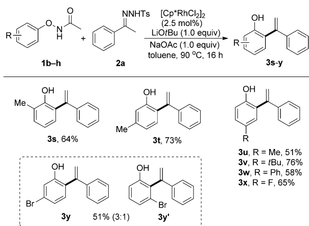
Scheme 4. Scope of N -phenoxyacetamides. Reaction conditions: 1b-h (0.30 mmol), 2a (0.30 mmol), [\text{Cp}^*\text{RhCl}_2]_2 (2.5 mol%), LiOtBu (1.0 equiv), and NaOAc (1.0 equiv) in toluene (3 mL) at 90 °C for 16 h.
